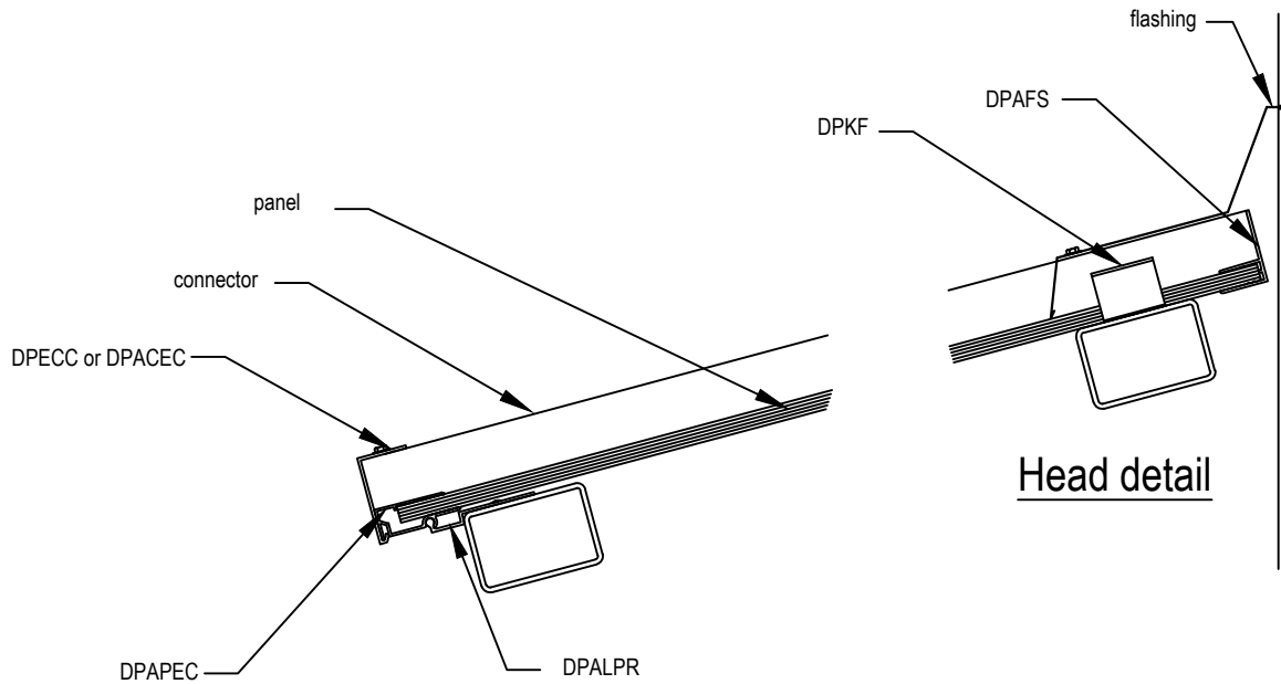
Purlin attachment
