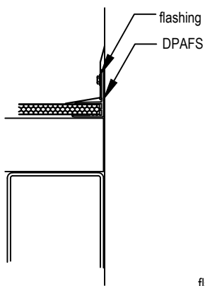
Wall detail
